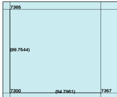
Figure 11: Finer Mesh in Main Column
