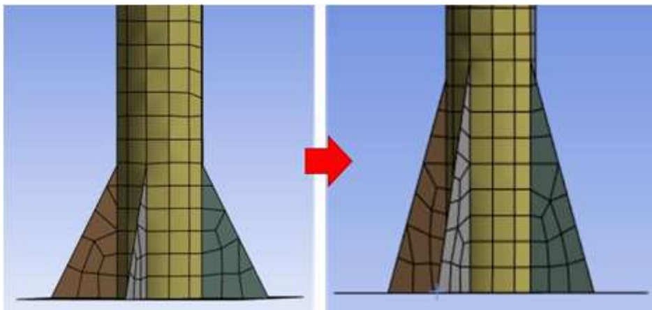
Figure 17: Increased Stiffeners Size
