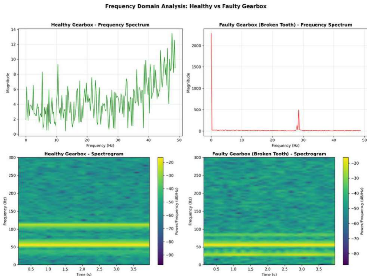
Figure 15: Frequency domain analysis showing FFT spectra and spectrograms for healthy and faulty gearboxes. The faulty gearbox shows additional frequency components and sidebands.
