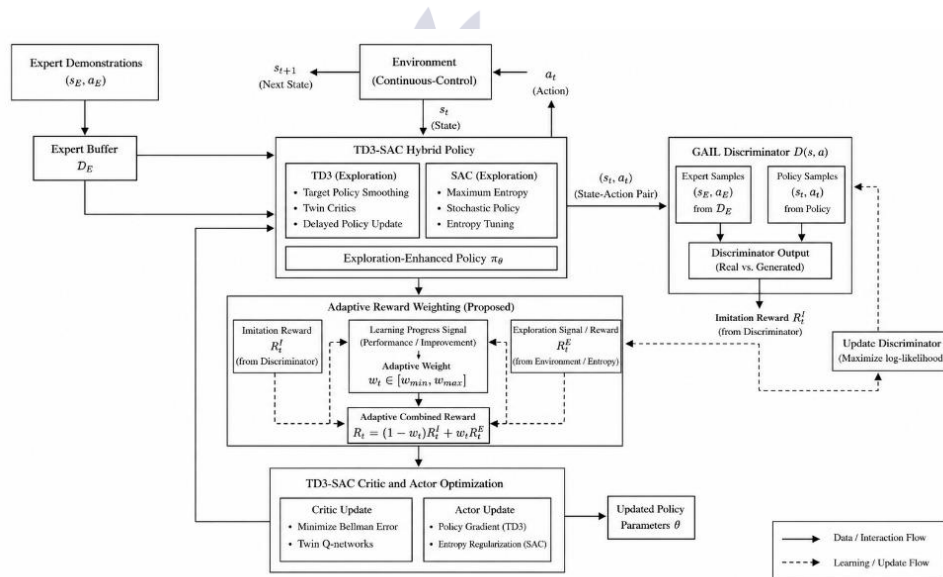
Fig. 1. Overall architecture of the proposed Adaptive TD3-SAC-GAIL framework with adaptive reward weighting for stable imitation learning.
