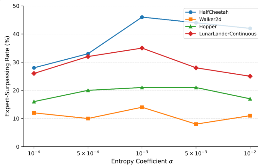
Fig. 3. Effect of the entropy coefficient \alpha on expert-surpassing performance across different environments.
