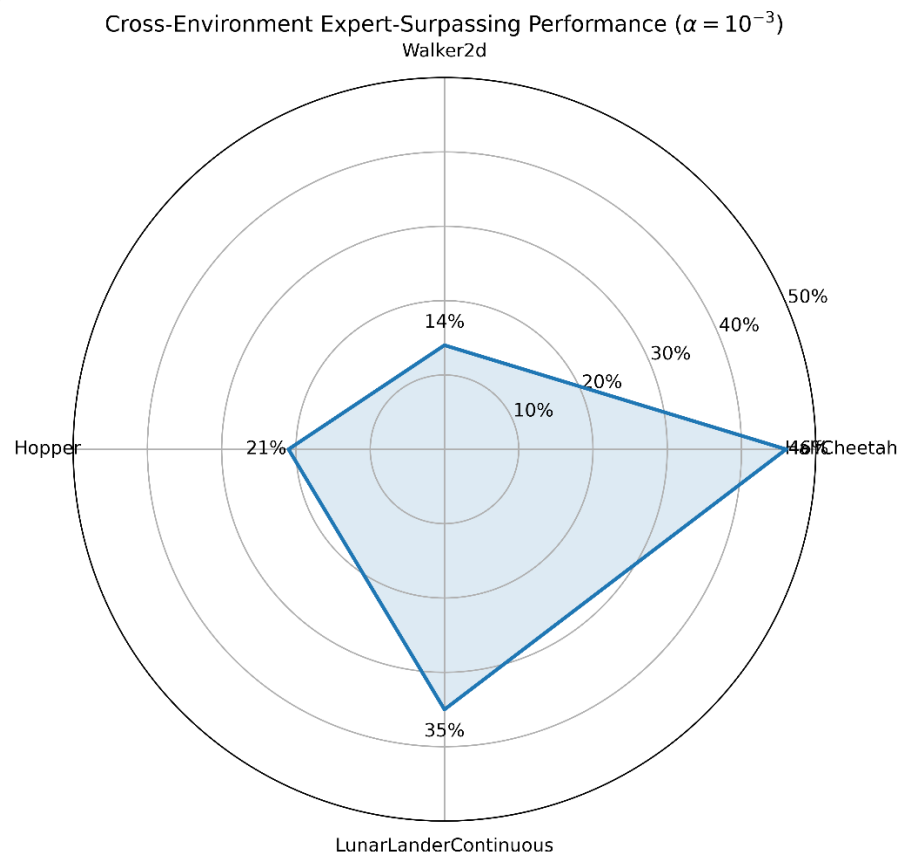
Fig. 4. Cross-environment expert-surpassing performance at \alpha=10^{-3} .
