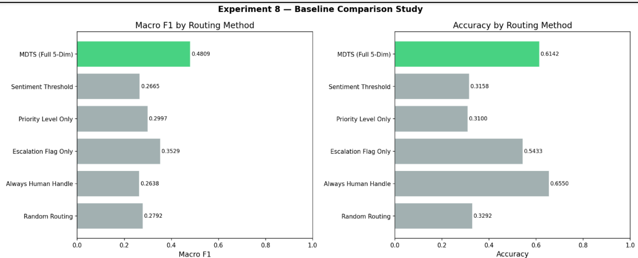
FIGURE 14. Baseline Comparison
