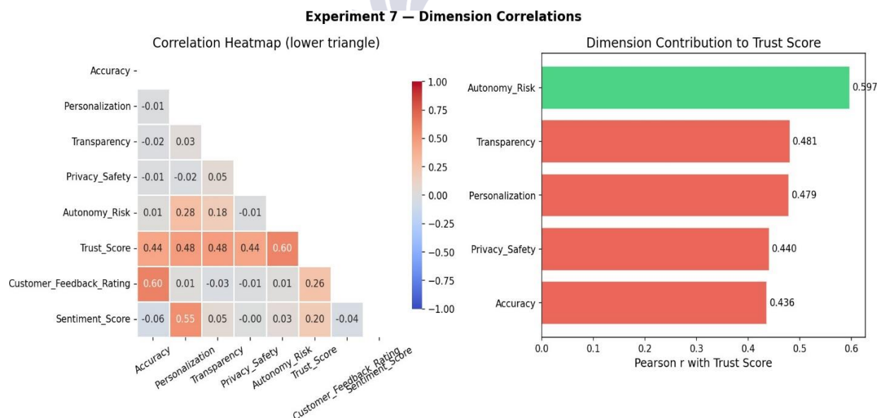
FIGURE 13. Dimension Correlations
