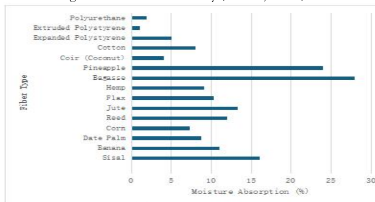
Figure 5: Comparative analysis of Moisture Absorption of Investigated Materials
