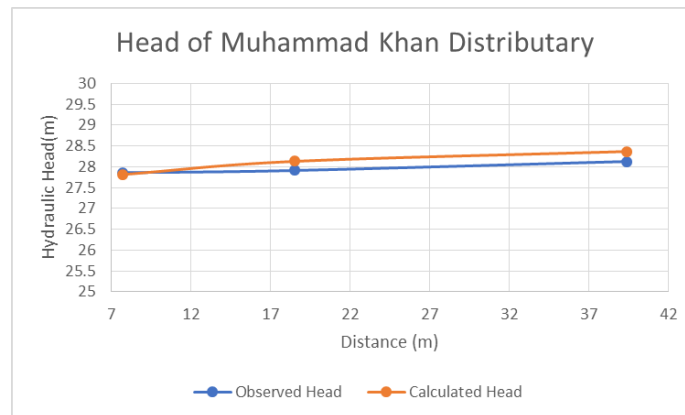
Figure 3: Hydraulic Head vs. Distance in 5 hours duration
