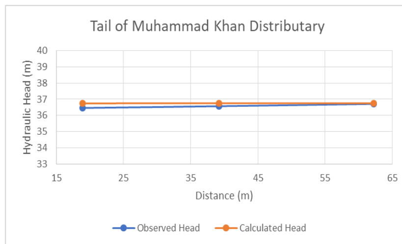
Figure 2: Hydraulic Head vs. Distance at 4.667 hours duration
