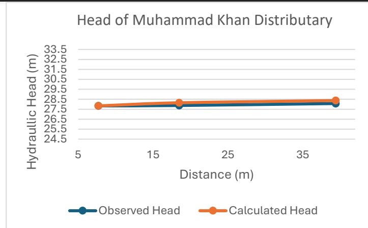
Figure 1: Total simulation period's division into stress periods for Head Tube-well
