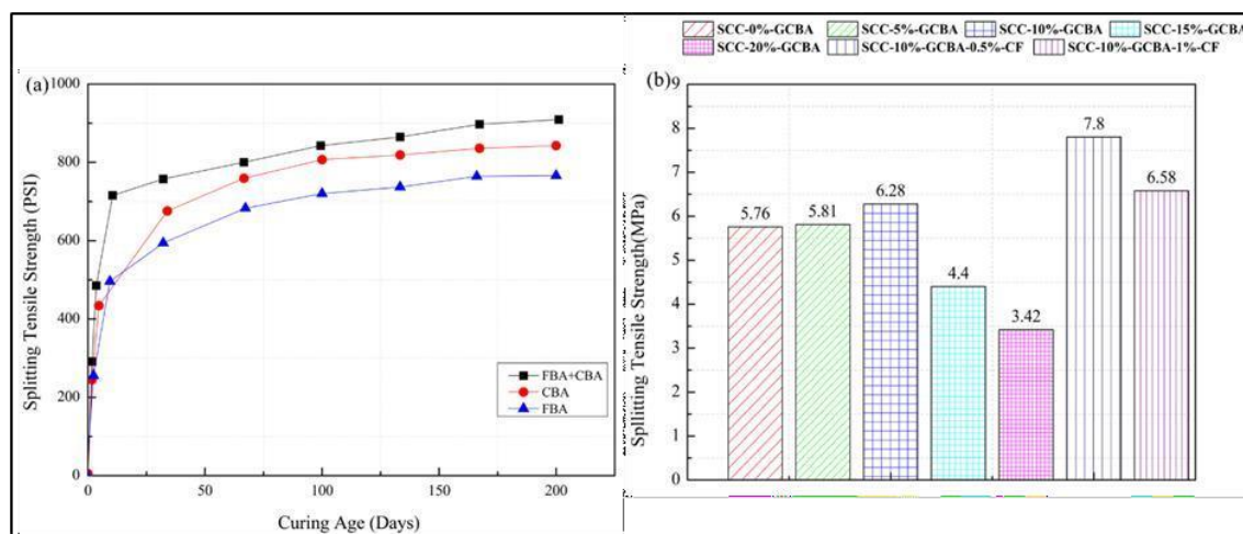
Figure 4: Relationship between curing age versus tensile strength of specimens; (a) Effect of curing age on splitting tensile strength; (b) Splitting tensile strength of different concrete matrixes.
