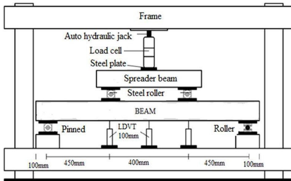
Figure 2: Experimental setup for flexural test
