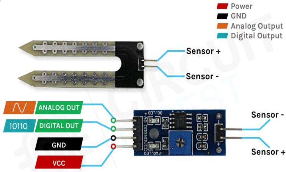
Figure 2: Moisture sensor
