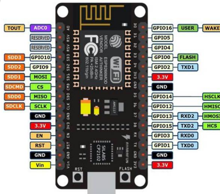
Figure 3: NodeMCU pinout
