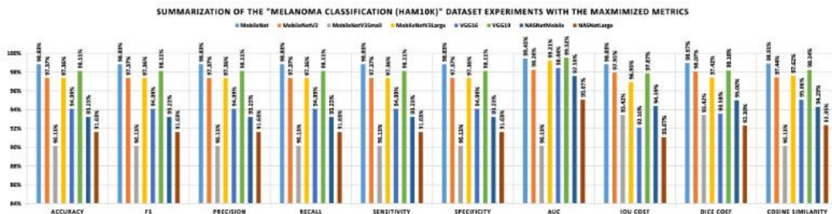
Graph 6 “Melanoma Classification (HAM10K)” dataset experiments with the maximized metrics
