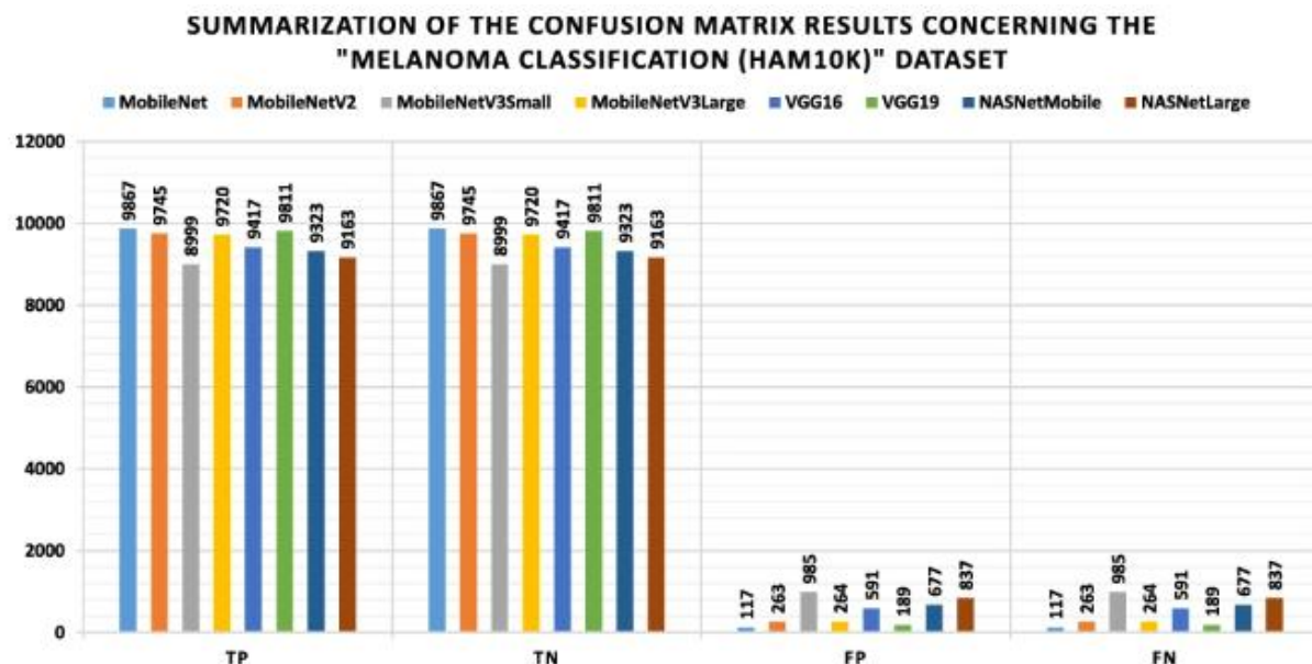
Graph 5: Confusion matrix results concerning the “Melanoma Classification (HAM10K)” Dataset
