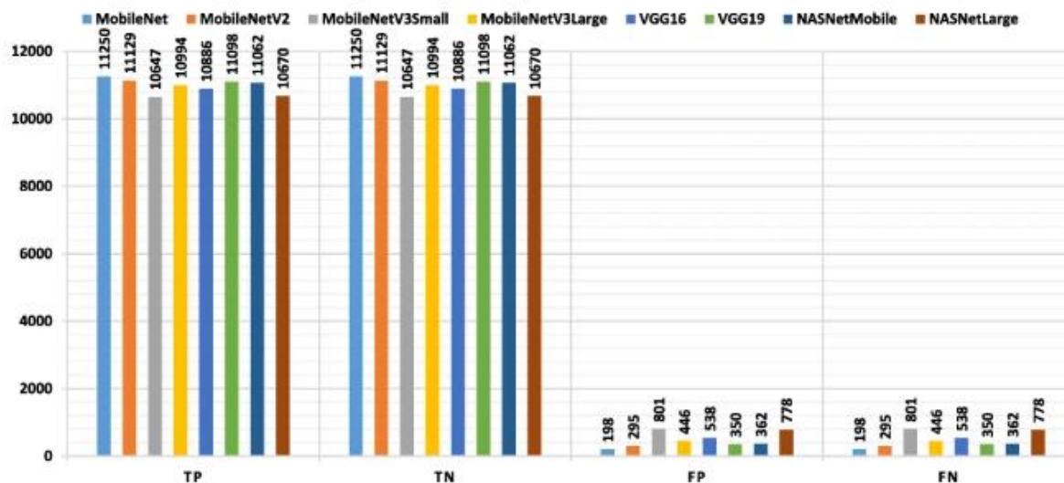
Graph 3: Confusion matrix result concerning the “ISIC 2019 and 2020 Melanoma dataset” dataset.
