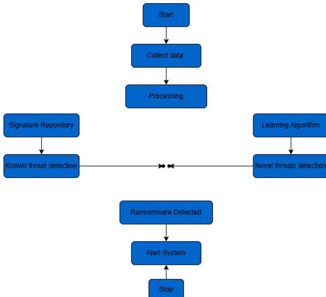
Figure 3.1 Dual level detection system Flow chart (self constructed)
