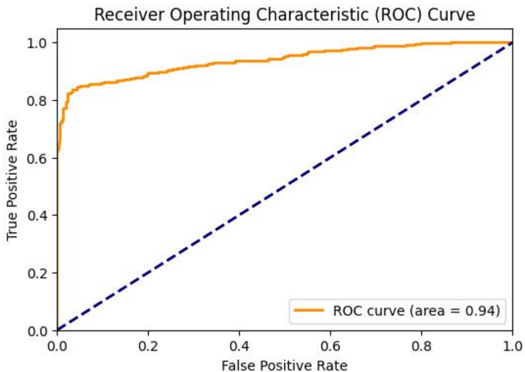
Figure 4.3 shows the ROC Curve with an AUC score of 0.94
