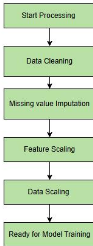
Figure 3.2 Data Pre Processing Steps (Self constructed)
