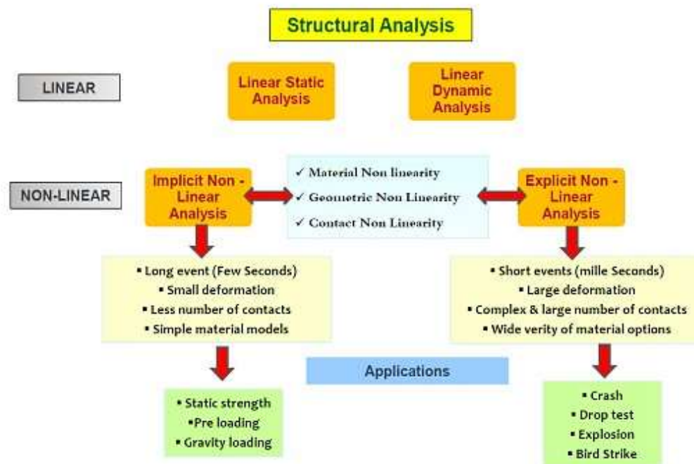
Figure 0-5: Static Structural Analysis in FEA
